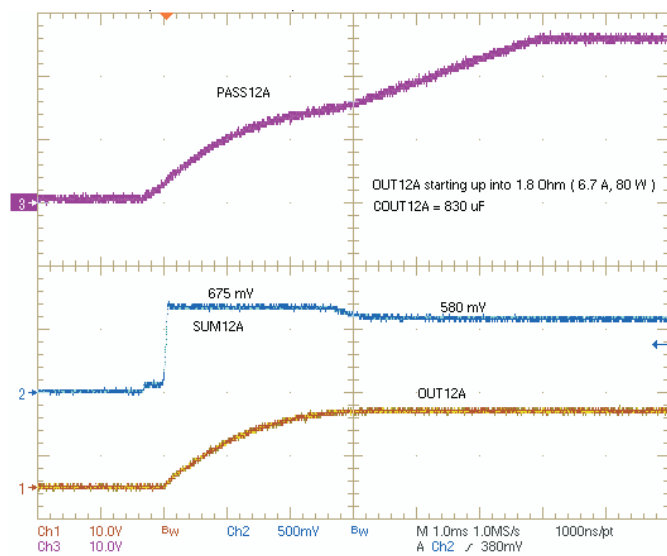
Figure 16. OUT12A Startup Into 80-Watt, 830-µF Load
