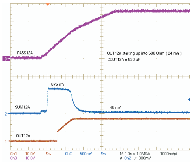
Figure 15. OUT12A Startup Into 500-Ω, 830-µF Load
